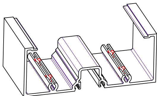
SF200-PROFILE
